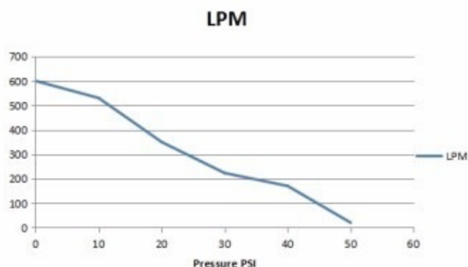
Characteristic Curve
