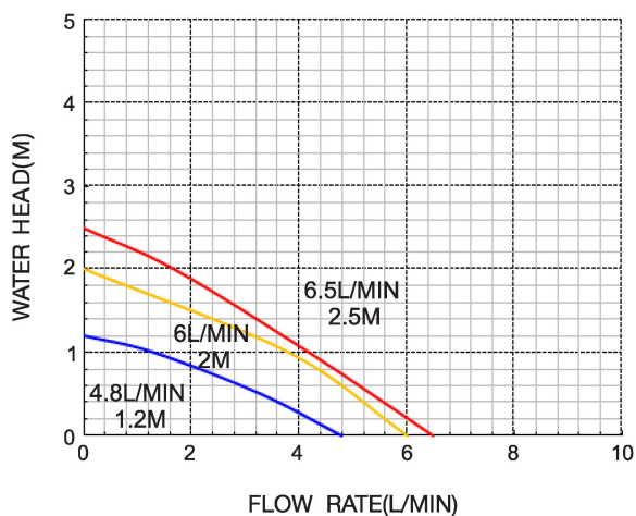
TL-B03 Performance
