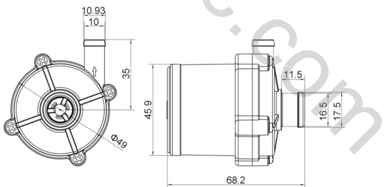
Dimension (mm)
